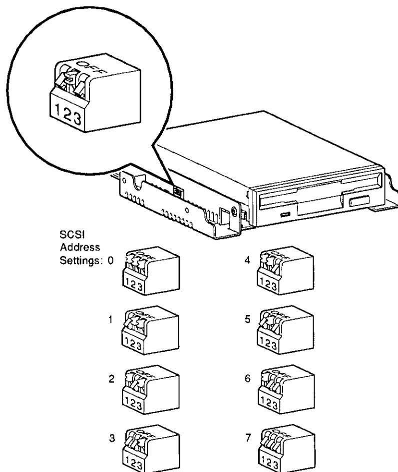
Figure 4-2 RX26 SCSI Address Switches
