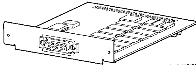
Figure 10-9 AUI Ethernet Module
