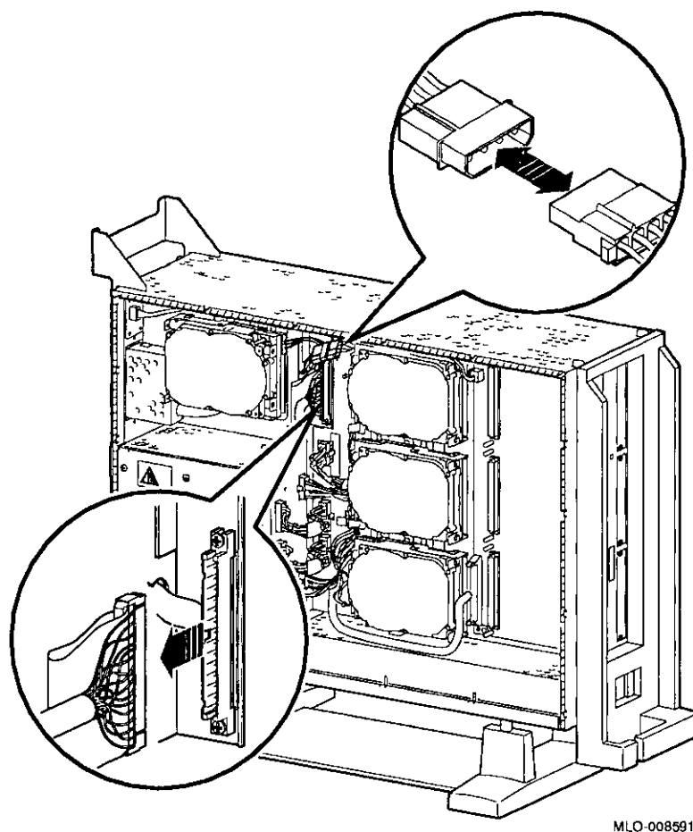
Figure 6-3 Disconnecting Bracket Power and SCSI Cables
