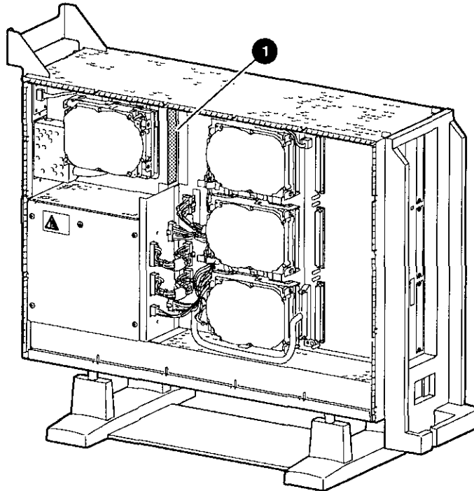
Figure 6–11 Bracket Power Cable Opening
