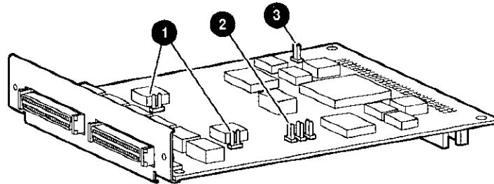
Figure 10-12 Dual SCSI Module Jumpers
