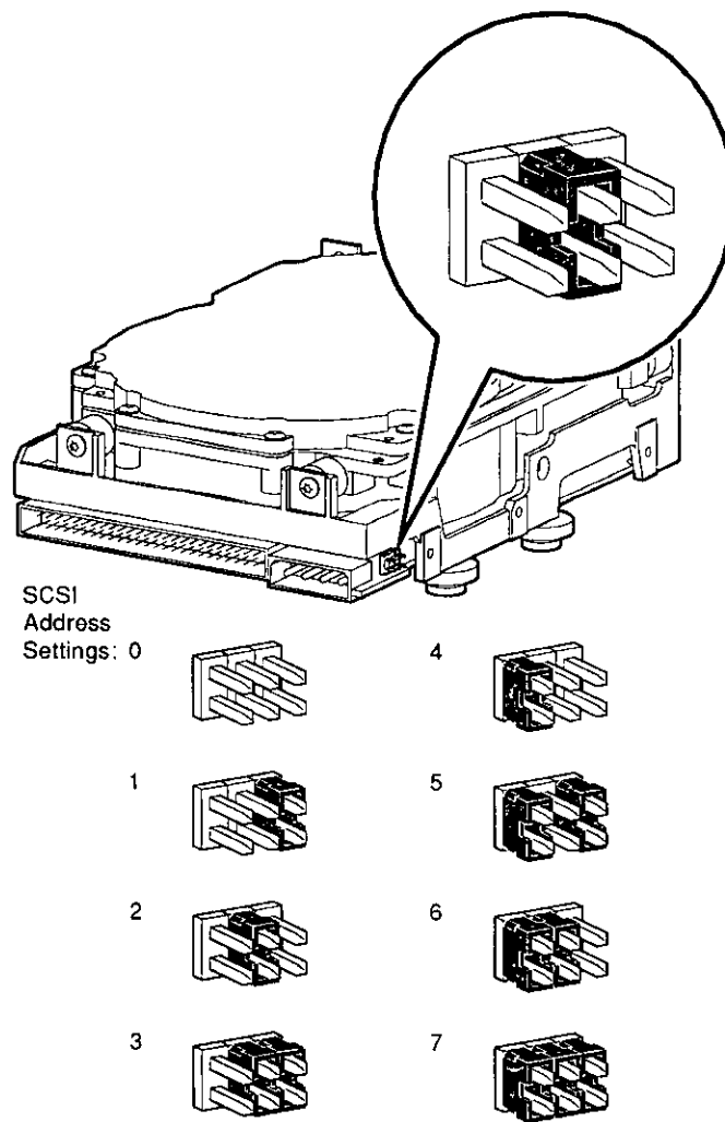
Figure 7-2 RZ25 SCSI Address Jumpers
