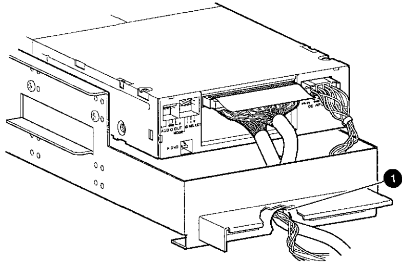
Figure 3-9 Slipping Cables into Slot
