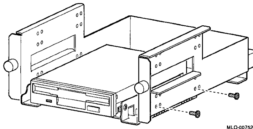
Figure 4-9 Placing the Drive into the Bracket
