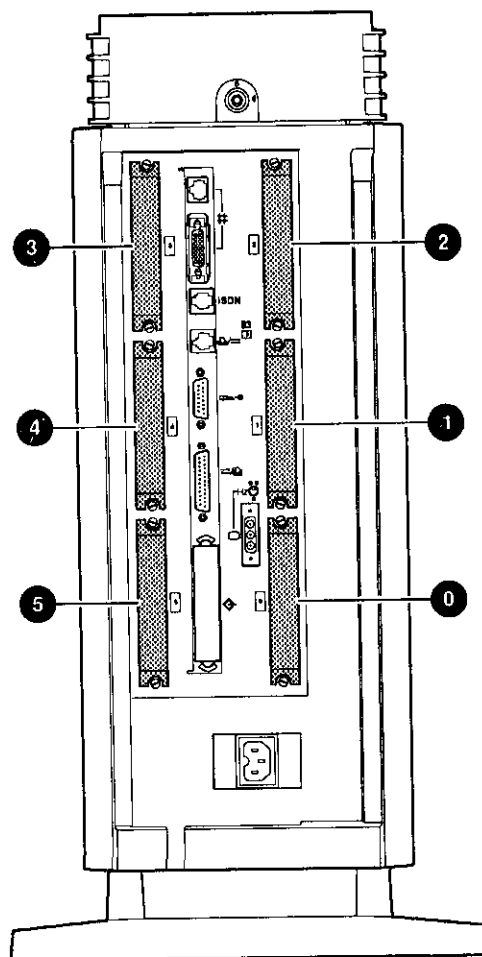
Figure 10-1 TURBOchannel Option Slots
