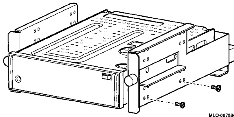
Figure 5-8 Placing the Drive Into the Bracket
