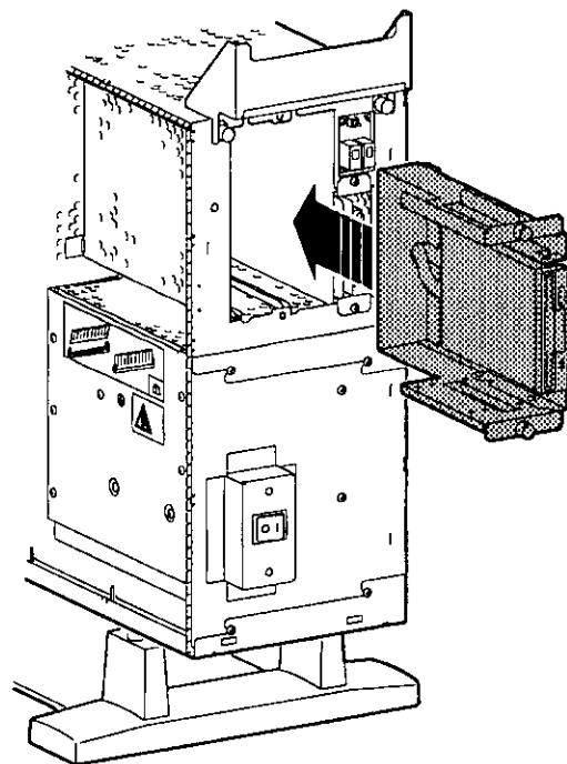
Figure 4-11 Sliding the Bracket Into the System
