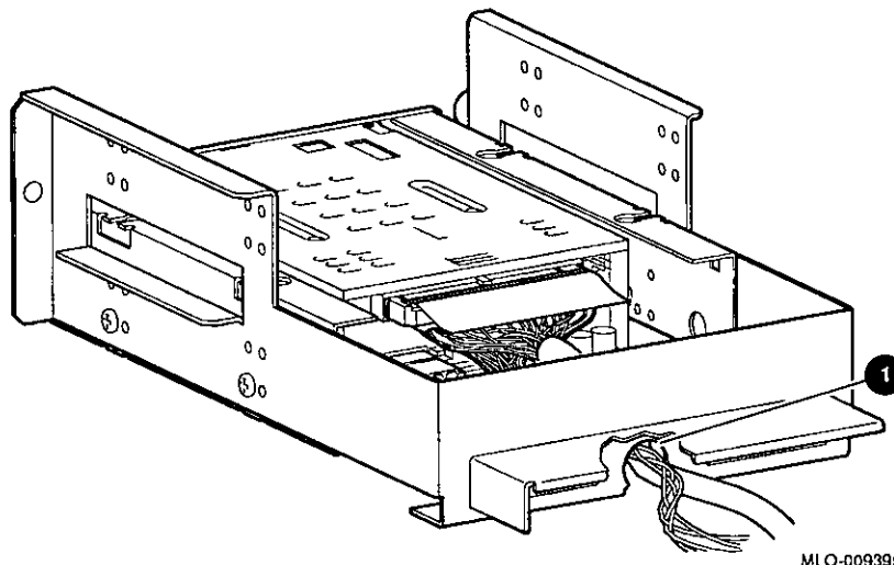
Figure 6-9 Slipping Cables into Slot
