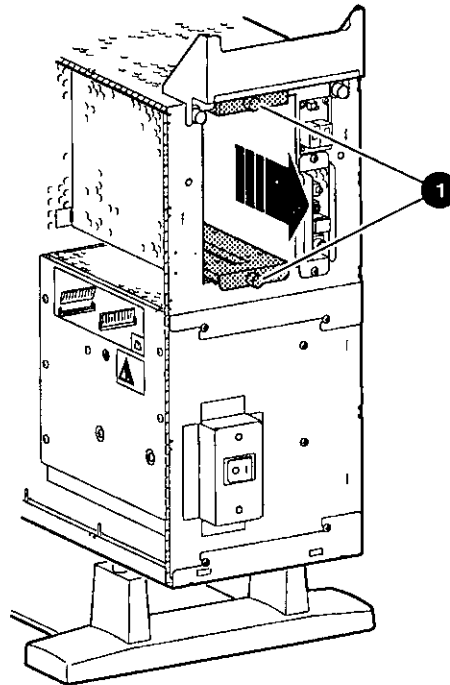
Figure 5-4 Removing the Drive Bracket
