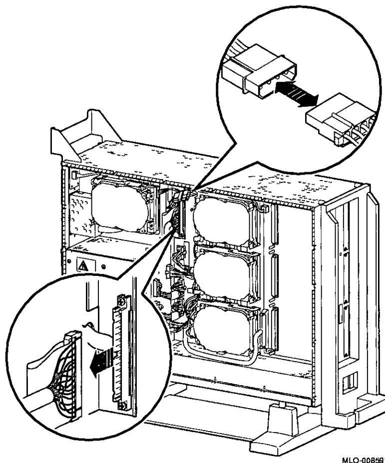
Figure 5-3 Disconnecting Bracket Power and SCSI Cables
