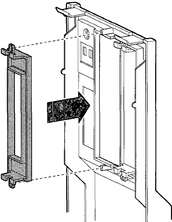
Figure 4-15 Placing the RX26 Bezel in the Front Panel
